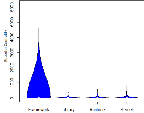
Figure 2. Centrality Bug Reporter Density - Android Layer Comparison
